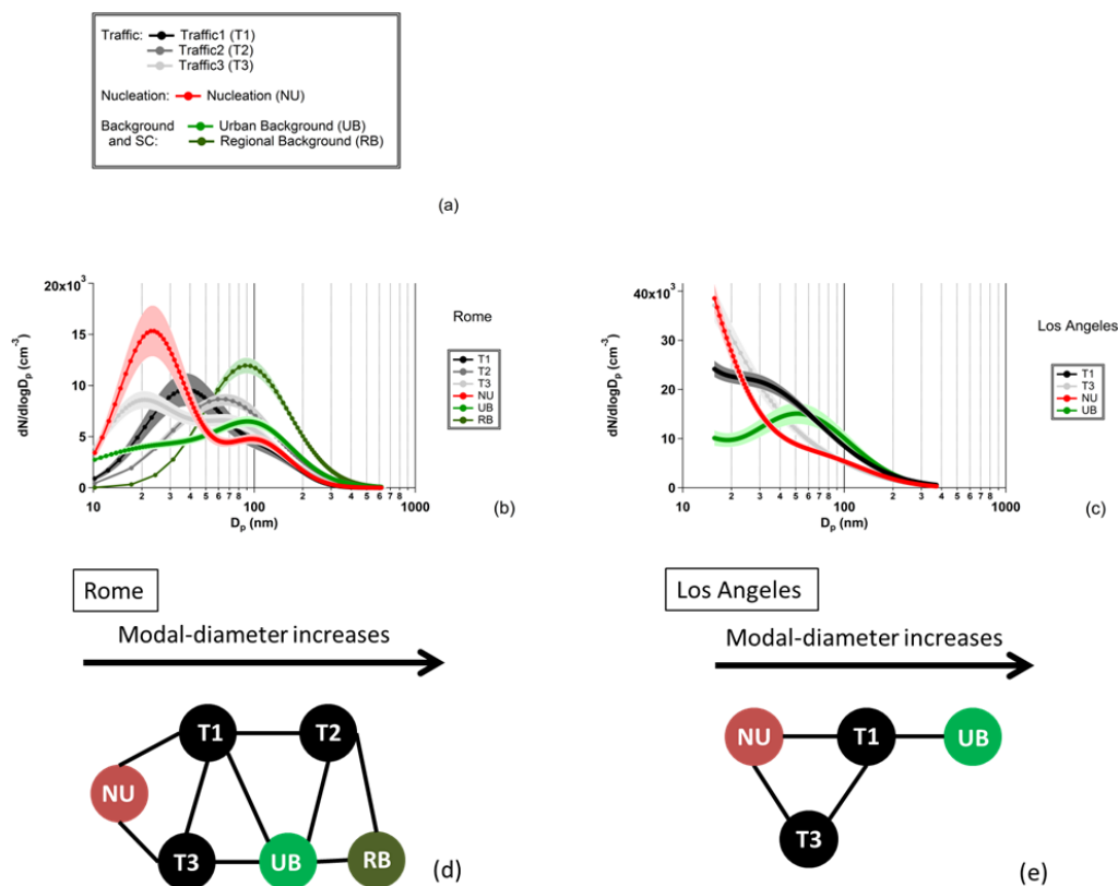
Figure 3. Aerosol size distribution results of the k -means cluster analysis performed on the SMPS data at the selected complementary cities: (a) legend, (b) Rome and (c) Los Angeles. Shaded areas around the curves represent the confidence limits calculated for 3\sigma . Please note the different scales for dN/d\log D_p . Cluster proximity diagrams are shown for both cities: (d) Rome and (e) Los Angeles.
