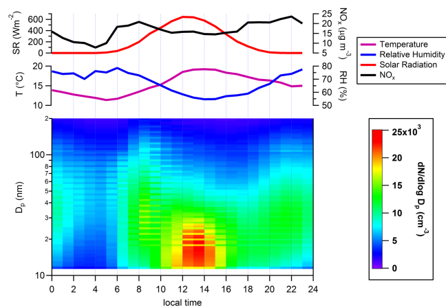
Figure 6. Daily average PN size distribution, temperature, relative humidity, solar radiation and \text{NO}_x levels on a nucleation day using data from Barcelona, Madrid and Brisbane.
