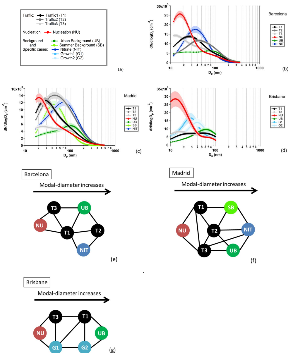
Figure 2. Aerosol size distribution results of the k -means cluster analysis performed on the SMPS data at each selected city: (a) legend, (b) Barcelona, (c) Madrid, (d) Brisbane. Shaded areas around the curves represent the confidence limits \mu calculated for 99.9 % confidence level. Please note the different scales for dN/d\log D_p . The corresponding cluster proximity diagram (CPD) is shown for the three main selected cities: (e) Barcelona, (f) Madrid and (g) Brisbane.
