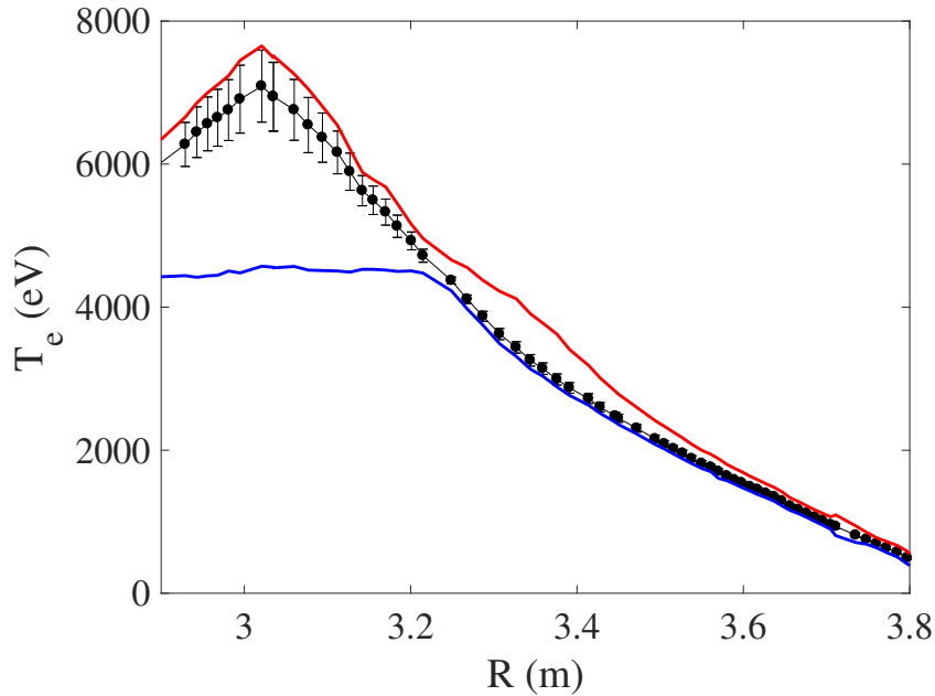
Figure 10. Black dots: ECE T_e -profile of a discharge of the power scan (90672), averaged over the time window of interest. The bars shown indicate the standard deviation of T_e in this time window, not its error. Upper continuous red line: maximum T_e ; bottom continuous blue line: minimum T_e over the time window.
