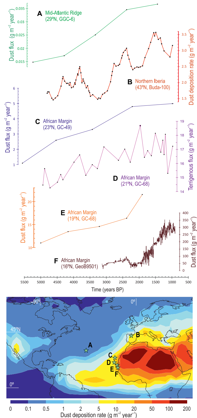
Fig. 3. Saharan dust in Iberia versus North Atlantic paleodust records. Dust reconstruction based in Buda-100 stalagmite compared with previous dust reconstructions based in marine sediment core GG-6 of the mid-Atlantic ridge (13) and sediment cores GC49 and GC68 (12), GeoB9501 (14), and ODP-658C (15) of the northwestern African margin. Beyond the different resolution of the records, all show good coherence in the long-term trend. Also, the absolute values of dust fluxes are concordant with the distance of the sampling sites to dust sources and pathways. The map shows current average dust deposition (32) rates and location of paleodust record sites.
