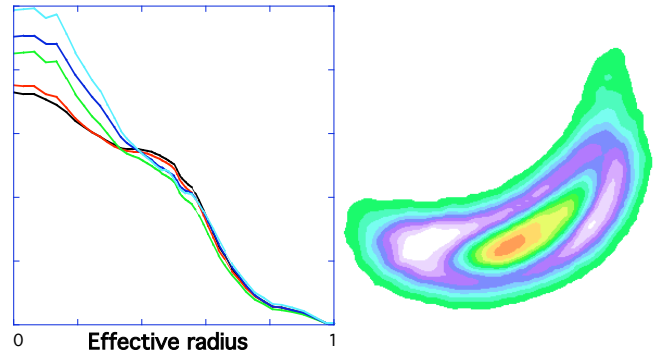
Figure 6 SXR profile evolution and difference between the tomographic reconstructions of the profiles before and after the transition. Results show a m=2 poloidal structure around \rho \approx 0.4 .
