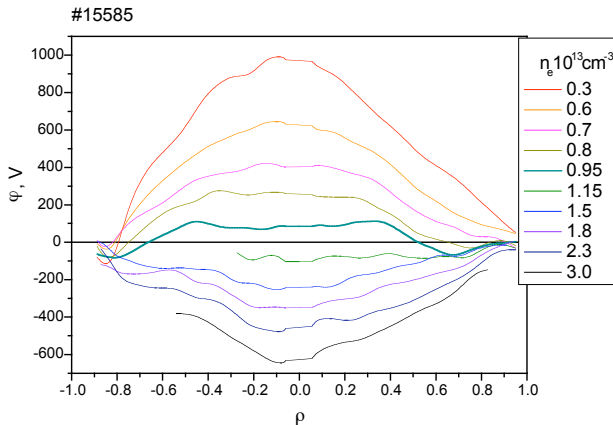
Fig. 1 Plasma potential profiles as density increases from the pure ECRH phase (red) to the ECRH+NBI one (grey).
