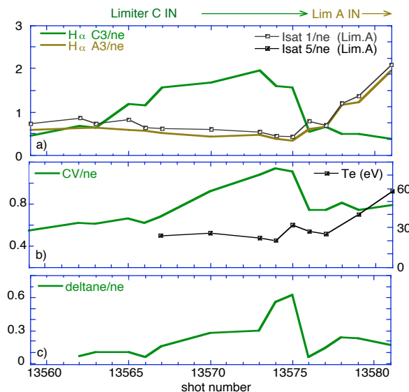
Fig. 13 Effects of limiter insertion in the plasma depending on hydrocarbon deposition. Limiter C, contaminated. Limiter A, clean
