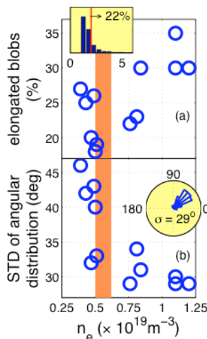
Fig. 8 During the development of spontaneous edge sheared flows, fluctuations in the angular distribution of blobs are reduced and the elongation of blobs increases.
