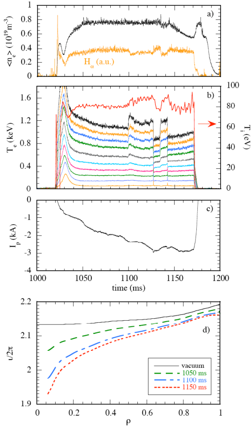
Figure 5 Time evolution of (a) line density and H_\alpha signal; (b) electron temperature at several radii and ion temperature measured along a central plasma chord; and (c) net plasma current, in a discharge with OH induction.
