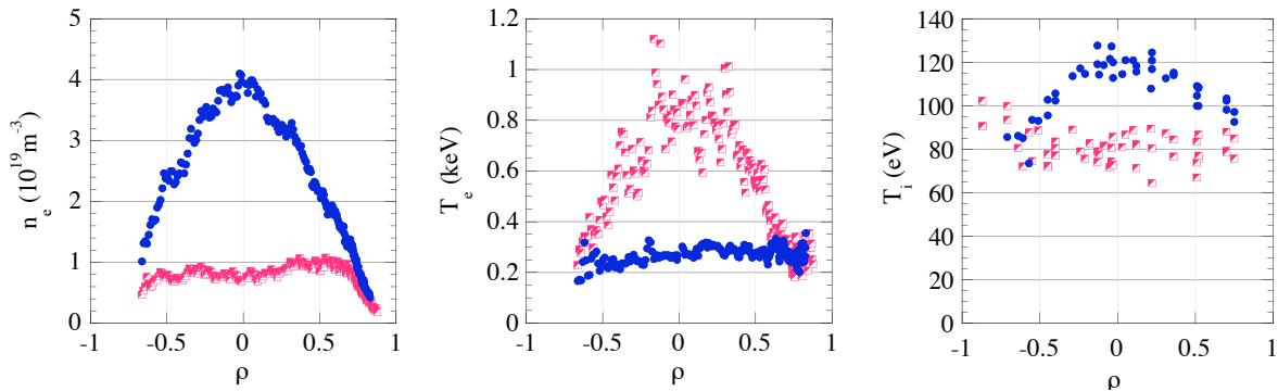
Figure 4: Density and electron and ion temperature profiles in ECH (red) and NBI (blue) plasmas
