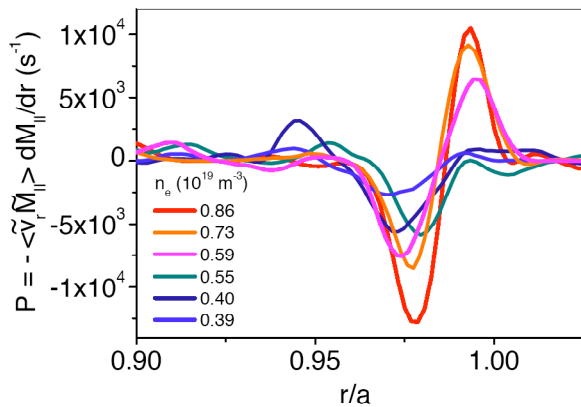
Fig.11 Parallel-radial component of the turbulence production term during edge sheared flow development in the TJ-II stellarator [4]. Evidence of significant energy transfer between turbulence and parallel flows at the on-set of sheared flows was found.
