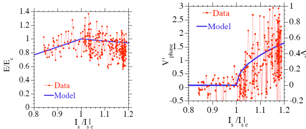
Fig. 9 Evolution of the level of turbulence (E) and averaged poloidal velocity shear from the model, in which the basic mechanism for the emergence of the shear flow is the Reynolds stress, and experimental results in the edge of TJ-II stellarator.
