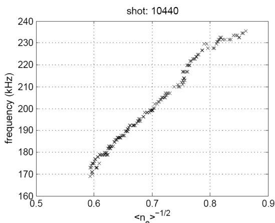
Fig. 12 Frequency vs. density in NBI plasmas
