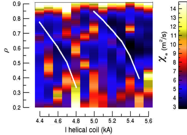
Fig. 5. (Left) Profiles of the effective electron heat diffusivity \chi_e for a configuration scan where the vacuum position (white lines) of the 8/5 (left) and the 5/3 (right) magnetic resonances is varied in normalized minor radius \rho . The abscissa shows the current in the TJ-II helical coil and is used as configuration label. (Right) Sequence in time of \chi_e -profiles in a discharge with increasing negative ohmic plasma current, which causes several magnetic resonances to move through minor radius as shown with lines.
