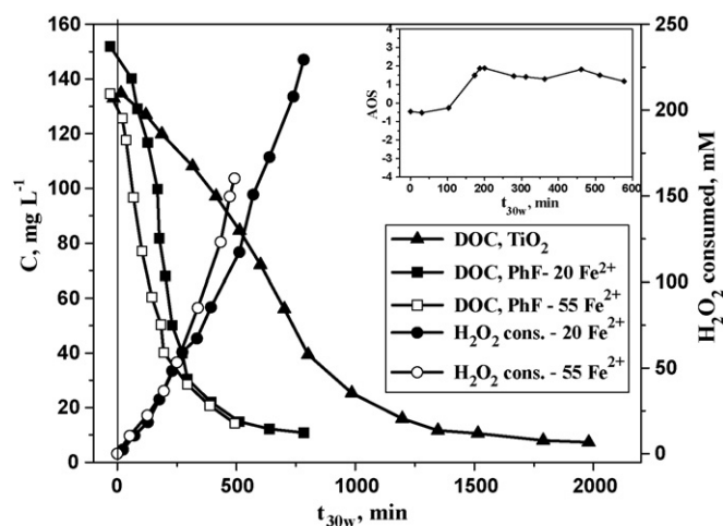
Fig. 2. Mineralization of the pesticide mixture by both AOPs and H 2 O 2 consumed during the photo-Fenton experiments. AOS evolution shown in figure inserted.
