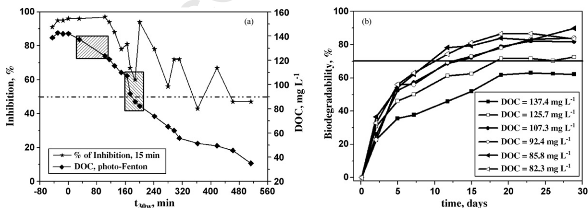
Fig. 3. (a) Percentage of Vibrio fischeri inhibition after 15 min exposure to samples partially treated by photo-Fenton at 20 mg/L of Fe 2+ . (b) Zahn-Wellens biodegradability analysis of photo-Fenton samples (labelled in (a)).
