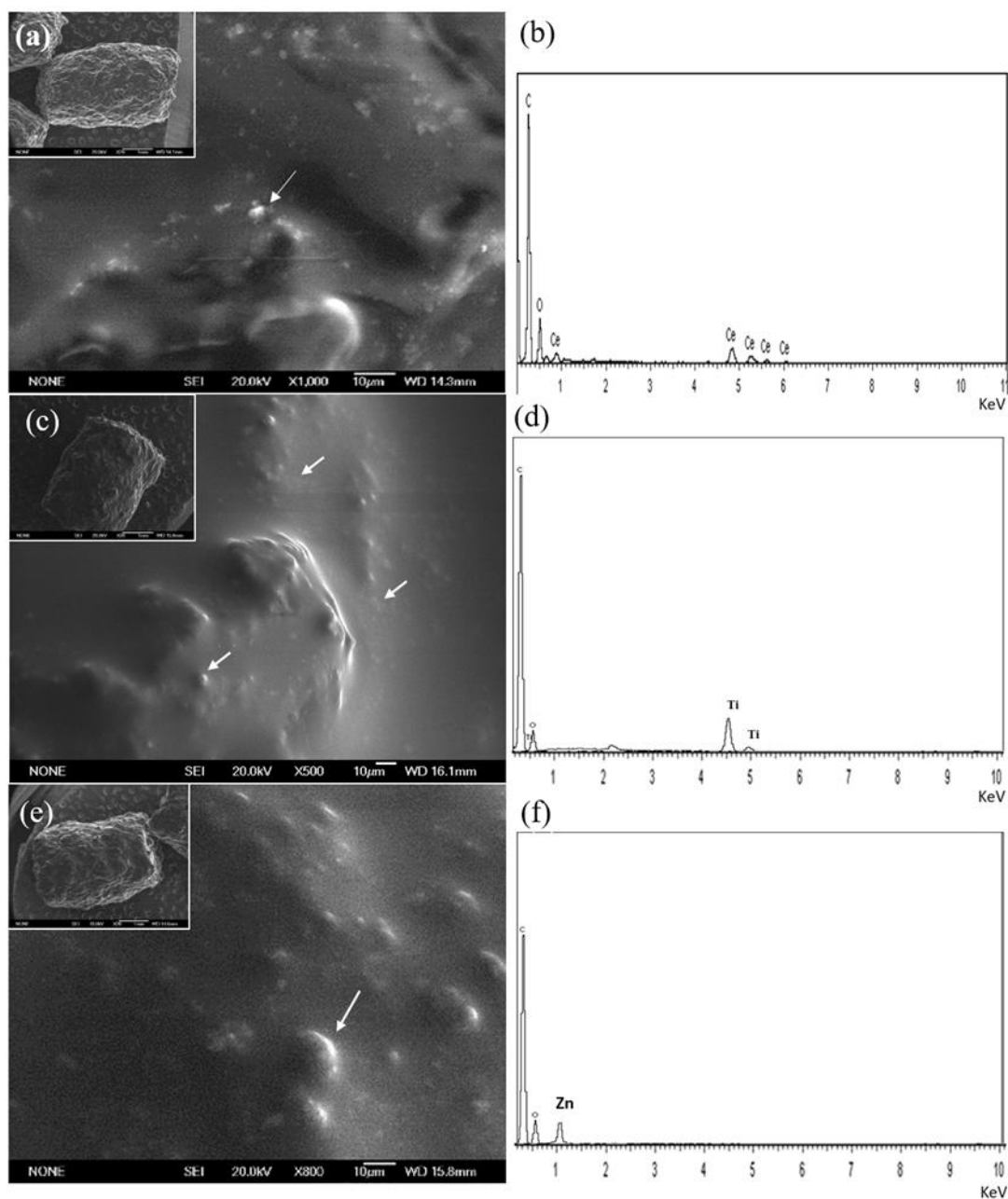
Figure S1. SEM micrographs of NP-sunflower oil dispersion soaked pellets along with respective EDX elemental analysis. Micrographs of \text{CeO}_2 NP soaked pellets (scale bars 1 mm and 10 μm) (a), and respective EDX analysis showing the presence of cerium on pellets (b). \text{TiO}_2 NP soaked pellets (scale bars 1 mm and 10 μm) (c) and EDX analysis showing the presence of titanium on pellets (d). \text{ZnO} NP soaked pellets (scale bars 1 mm and 10 μm) (e) and EDX analysis showing the presence of zinc on pellets (f).
