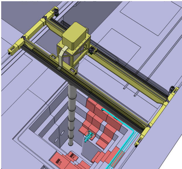
Fig. 18 ACME with its telescopic mast operating inside the TC
