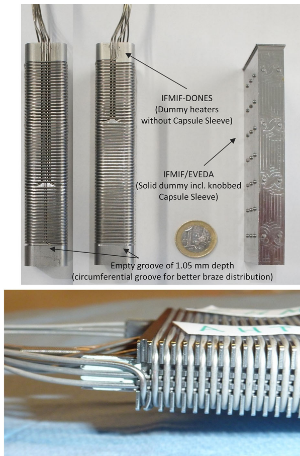
Fig. 24 HFTM capsule prototypes with electric heaters
