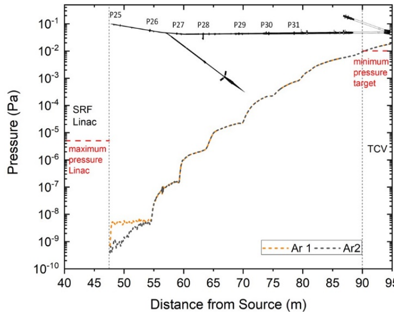
Figure 2. Pressure profile along HEBT (Case Ar1 + 2).
