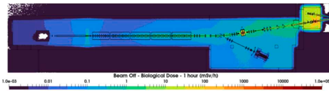
Fig. 6. Biological dose ( \text{mSv/h} ) at 1 h of cooling time in the AS room.
