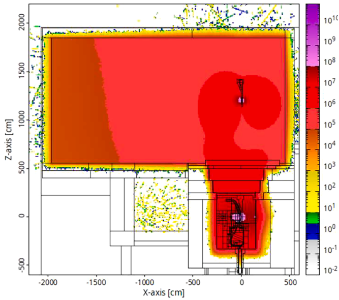
Fig. 16. Shutdown dose rate ( \mu\text{Sv/h} ) during TC opened and HFTM transportation after 345 days of operation and 1-day cooling.
