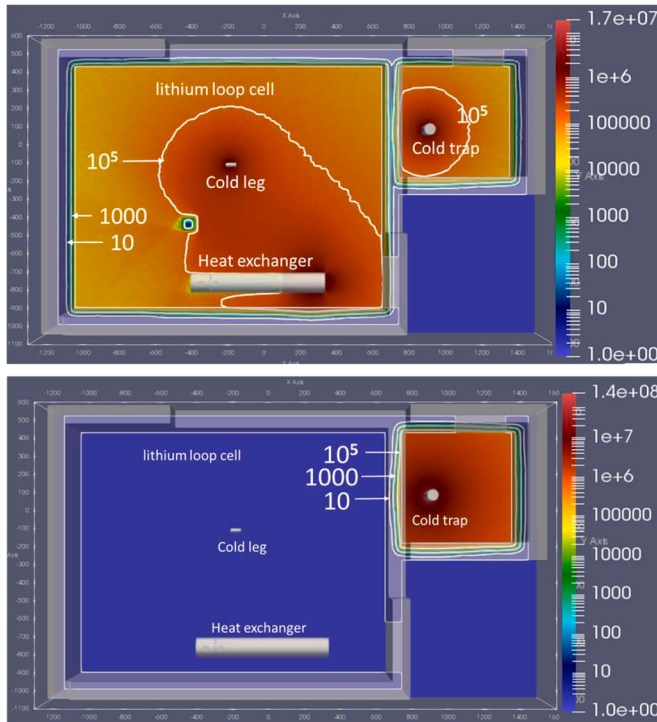
Fig. 14. Radiation dose map ( \mu\text{Sv/h} ) contributed by ^7\text{Be} during operation. Top – under operation temperature of 250^\circ\text{C} , and bottom – under 300^\circ\text{C} .
