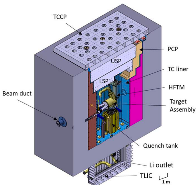
Fig. 7. Geometry of the TC and internal components.
