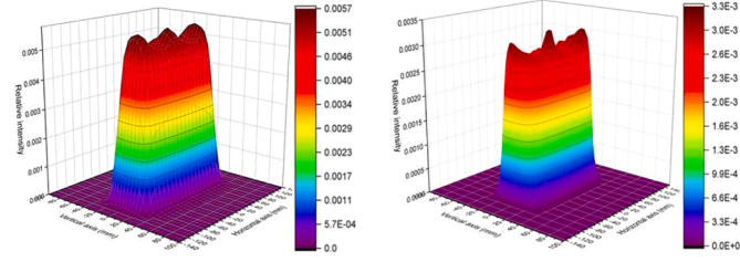
Fig. 9. The IFMIF/EVEDA 20 \times 5 \text{ cm}^2 beam profile (left) and the validated profile with a center-peak (right).
