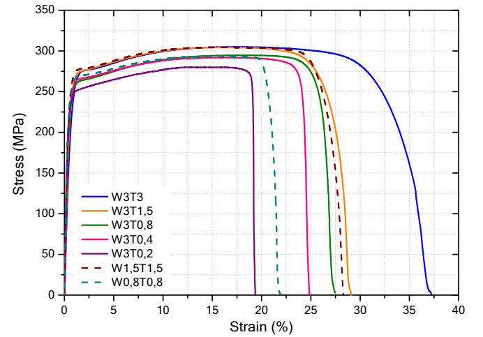
Fig. 3. Average stress–strain curves for specimen tested.
