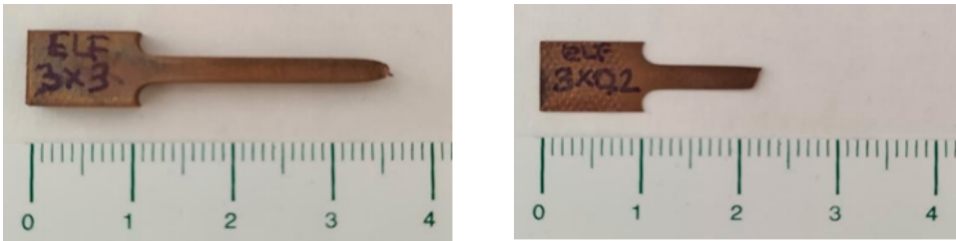
Fig. 4. Pictures of specimens tested, W3T3 (left) and W3T0.2 (right).
