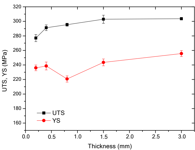
Fig. 7. Comparison of total UTS and YS of specimens tested W3 type with same width but different thickness.
