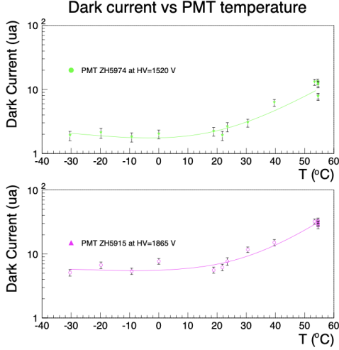
Figure 4: The PMTs response as a function of the temperature, superimposed is a parabolic fit.
