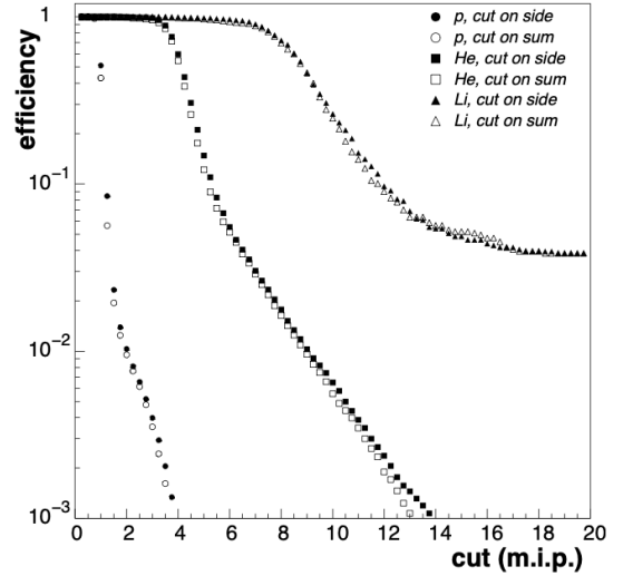
Figure 9: Trigger efficiency for different particles, as function of the threshold applied on the energy lost measured by a single counter side or by both ends.
