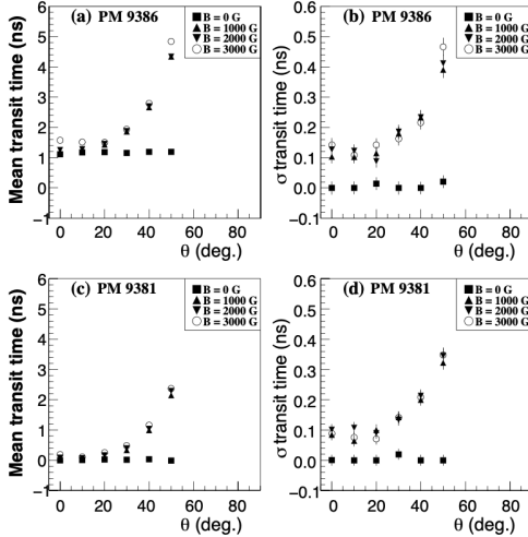
Figure 2: Magnetic field effect on the time measurement.
