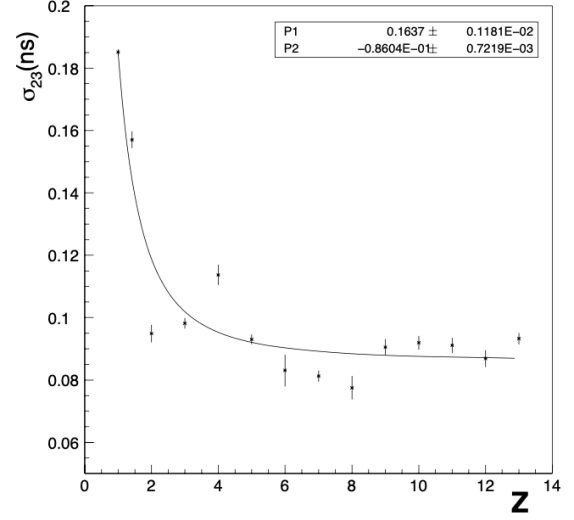
Figure 8: Resolution on the time of flight between C2 and C3 as function of the particle charge.
