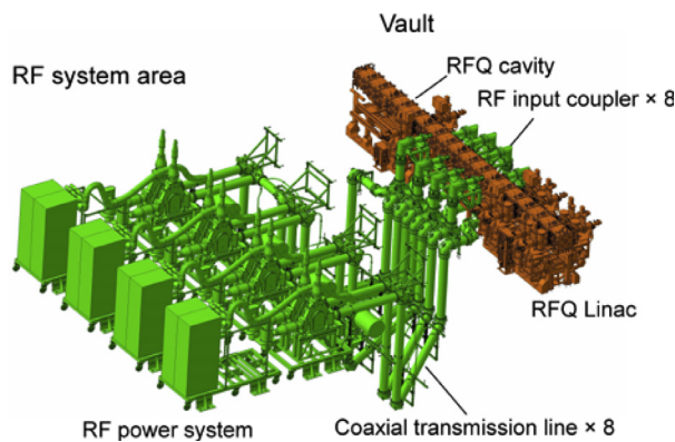
Fig. 8. 3D-model of the eight coaxial transmission lines connecting the RF power system in the RF system area to the RFQ Linac in the vault.
