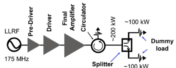
Fig. 7. Schematic of the high power test setup [15].
