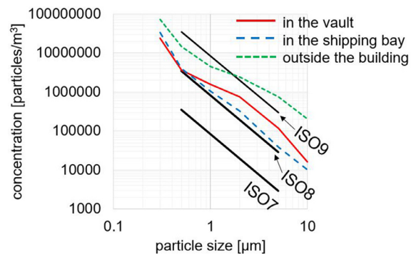
Fig. 3. The average cleanliness in the vault (solid line), shipping bay (dashed line), and outside the building (dotted line), measured in July - September 2016.
