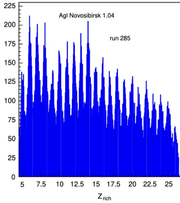
Figure 7: Charge reconstruction for n = 1.04 CIN Aerogel.
