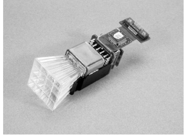
(b) One PMT module with light guide, electronics and half plastic shell.
