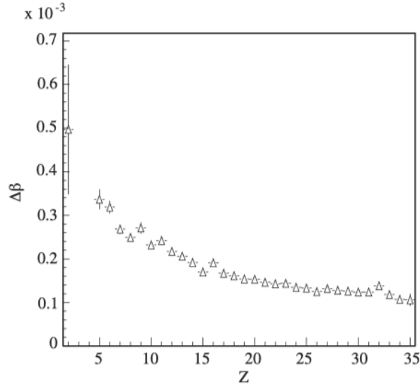
Fig. 7. Velocity resolution vs. charge.
