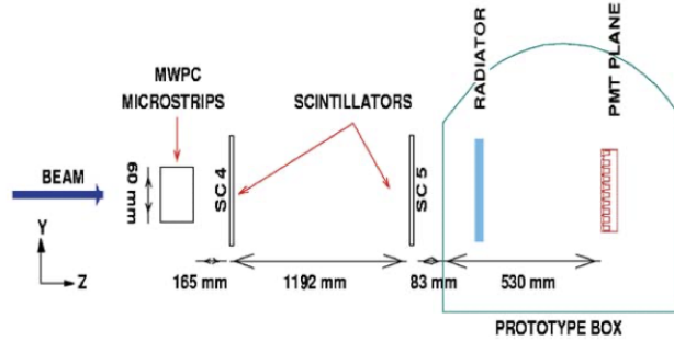
Figure 3: Experimental setup on the beam line.
