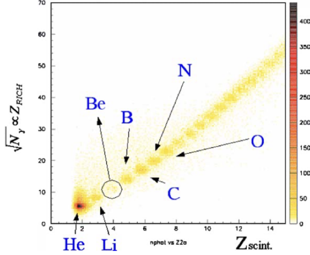
Figure 4: Correlation between a dE/dX scintillator and the square root of the number of Cherenkov photons.
