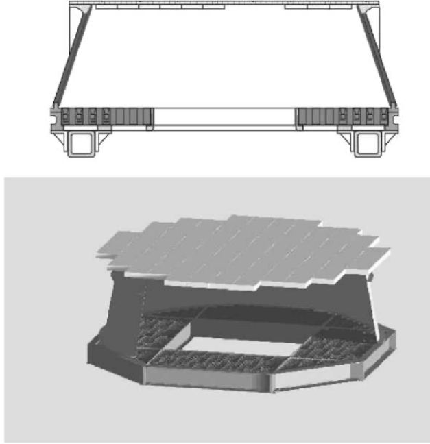
Figure 1: Structure of the final imager.
