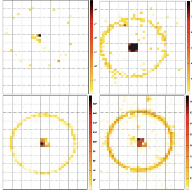
Figure 5: Ring patterns for Z = 2 (top left), 6 (bottom left), 10 (top right) and around 26 (bottom right).
