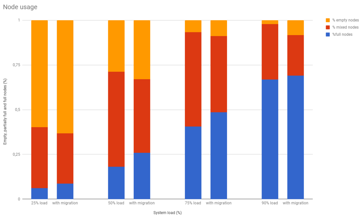
Figure 4. Cluster state with different workloads. Execution time is one day.
