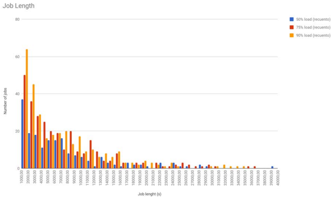
Figure 2. Distribution of the job length in the workloads depicted in Fig. 1.
