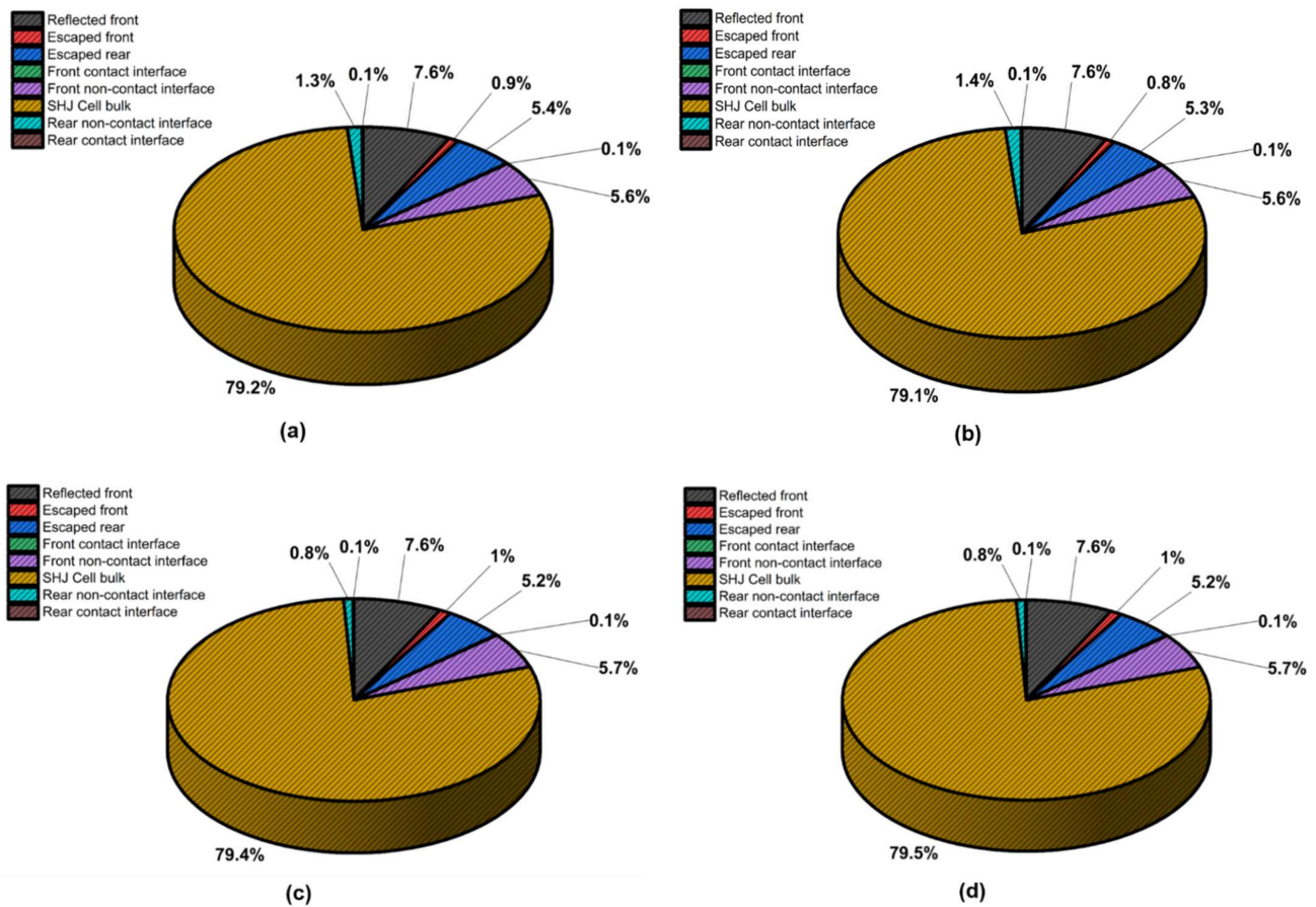
Figure 5. Pie charts represent optical current density in SHJ cell using MoS 2 as back-reflector layer for various structure: (a) SHJ; (b) SHJ/MoS 2 (1 nm)/ITO (70 nm)/Ag; (c) SHJ/MoS 2 (1 nm)/ITO (30 nm)/Ag; and (d) SHJ/ITO (30 nm)/MoS 2 (1 nm)/Ag.
