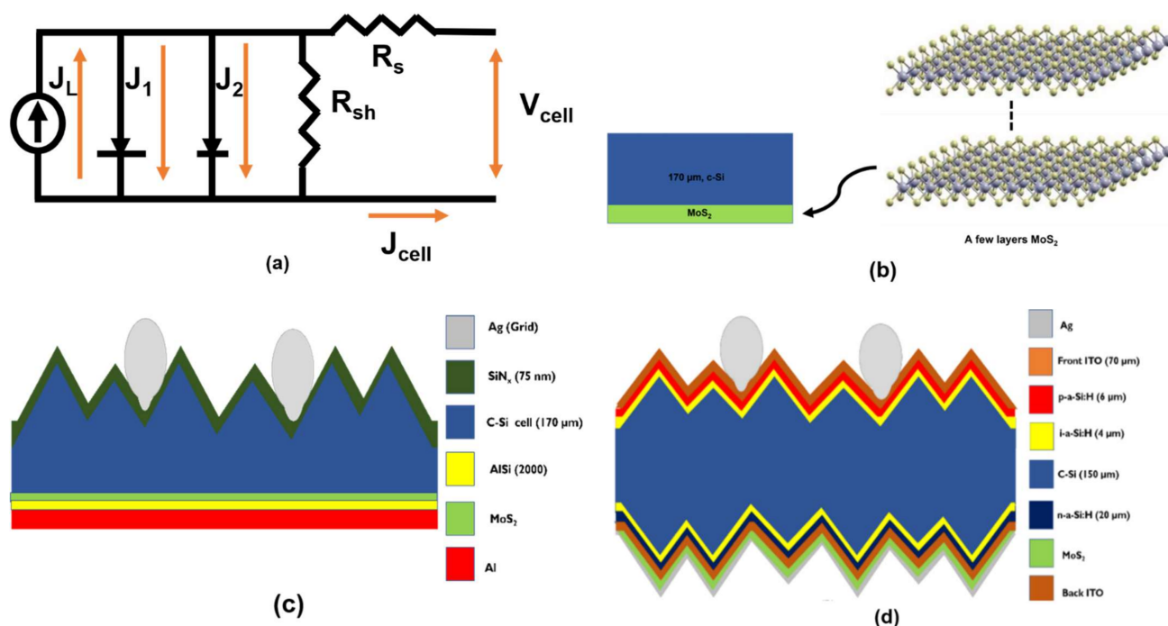
Figure 2. (a) Sunsolve electrical equivalent circuit model, (b) silicon wafer along with MoS 2 few layers at the backside, (c) SSP solar cell and (d) SHJ solar cell. (All figures not to scale).
