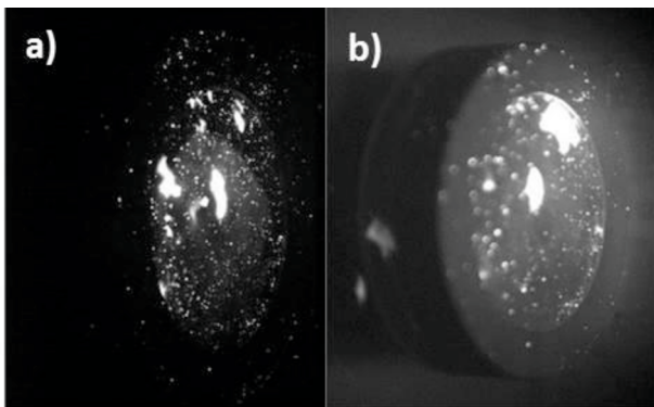
Fig. 9. Fast camera results for (a) 10MW/m 2 and 100 ms pulse (first day of operation with target) and (b) 8MW/m 2 and 50 ms pulse (last day of operation with target).
