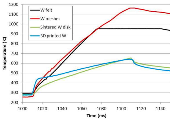
Fig. 16. Comparison of the temperature increment measured by the pyrometer for the four different Sn wetted W CPS subjected to a 100 ms long pulse producing 15 MW/m 2 on a target with 280 °C initial temperature (in the W felt case the pyrometer saturates at 1075 ms).
