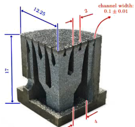
Fig. 5. Section of the 3D printed W target [10].
