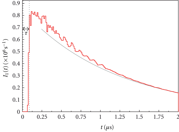
FIGURE 6: Example of the distribution of intervals between consecutive counts obtained from the Yalina-Booster experiments. Gray line represents the fit to a exponential (over a large range than the plotted interval).
