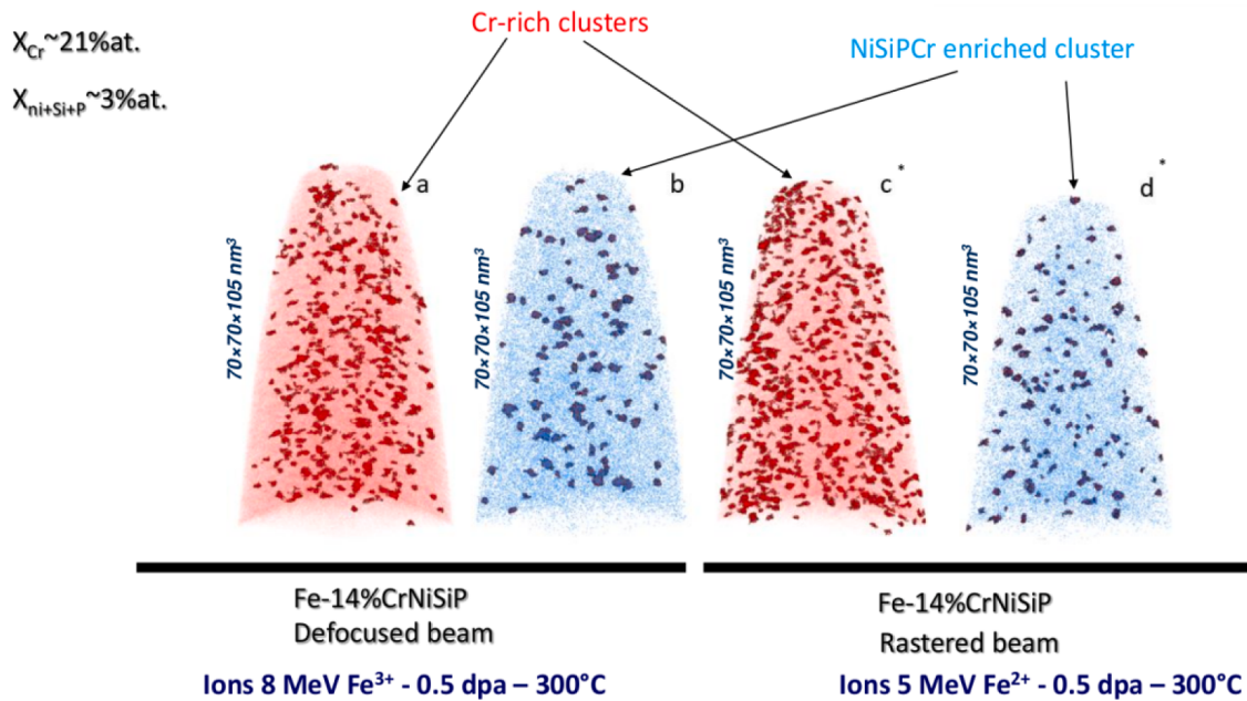
Fig. 15. APT results for two different irradiation conditions: (left) 8 MeV Fe and defocused beam (right) 5 MeV Fe and rastered beam, both to 0.5 dpa.
