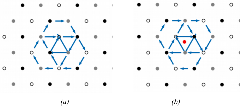
Fig. 19. Easy (a) and hard (b) cores relaxed with DFTB in pure iron and in presence of C atoms respectively. In (b) we recover the reconstructed prismatic core identified by DFT in [154].
