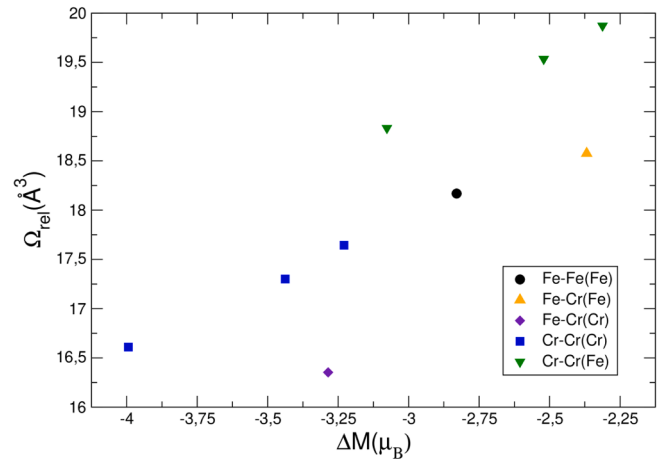
Fig. 5. The relaxation volumes of dumbbells in bcc Fe matrix as functions of the change in the magnitude of the total magnetic moment in the supercell associated with the formation of the defect [60].
