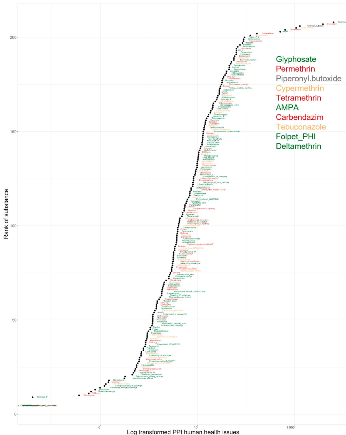
Fig. 9. Pesticide Prioritization Indicator (PPI) for humans. Residues are sorted from lowest to highest PPI values. The name of pesticide residues in red indicates not approved compounds, orange denotes candidates for substitution and green indicates approved compounds. The list on the top right corner corresponds to the 10 compounds with the highest PPI values. (For interpretation of the references to colour in this figure legend, the reader is referred to the web version of this article.)
