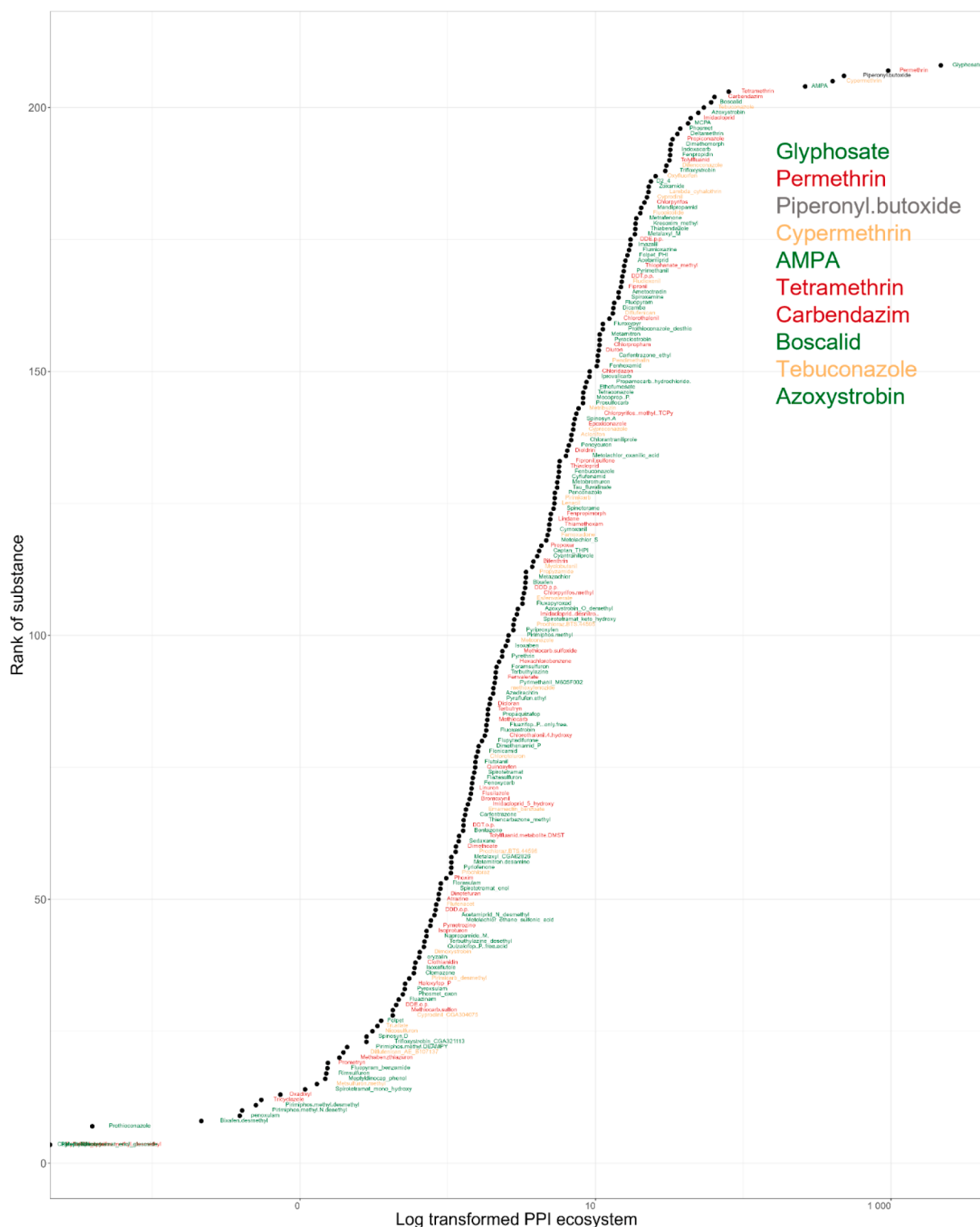
Fig. 8. Pesticide Prioritization Indicator (PPI) for ecosystems. Residues are sorted from lowest to highest PPI values. The name of pesticide residues in red indicates not approved compounds, orange denotes candidates for substitution and green indicates approved compounds. The list on the top right corner corresponds to the 10 compounds with the highest PPI values. (For interpretation of the references to colour in this figure legend, the reader is referred to the web version of this article.)
