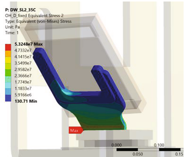
Fig. 16. OH2 maximum primary stresses in LCIV.1.
