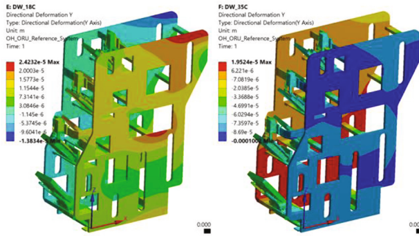
Fig. 18. Y deformation (m) in normal operation at 18 °C (left) and 35 °C (right).
