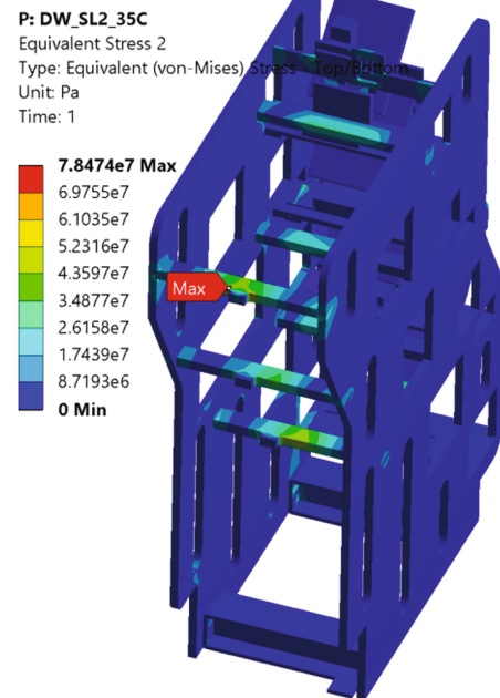
Fig. 13. Structure primary stresses in LCIV.1.
