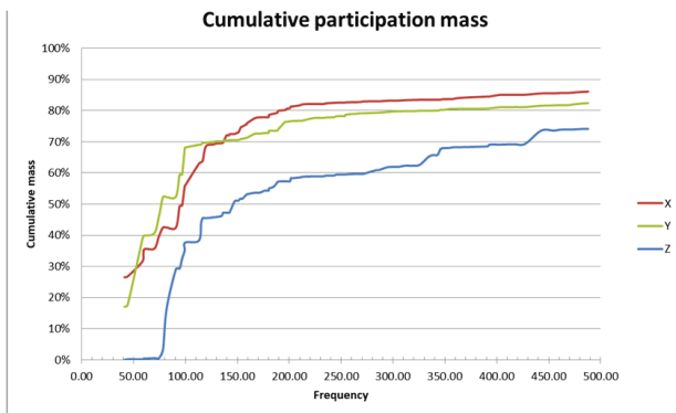
Fig. 12. Cumulative participation mass evolution for modal analyses in each direction.
