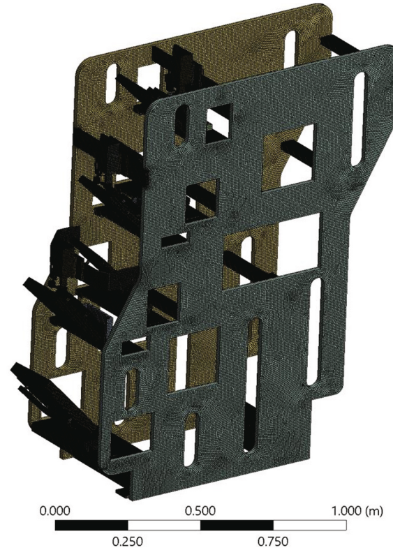
Fig. 9. FE mesh overview.
