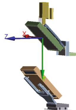
Fig. 4. LoS coordinate systems (decentering).
