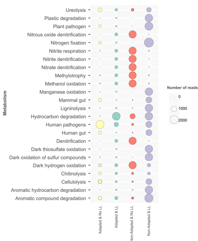
Figure 9. Main representative metabolisms in microbial communities from adapted and non-adapted compost samples before (no LL) and after (LL) being exposed to raw LL. The diameter of the circles represents the prevalence of each metabolism in the sample.
