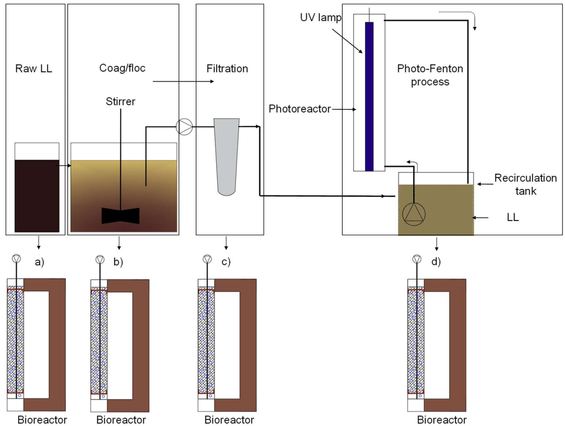
Figure 3. Schematic diagram of the pretreatment processes and final airlift packing bioreactors.
