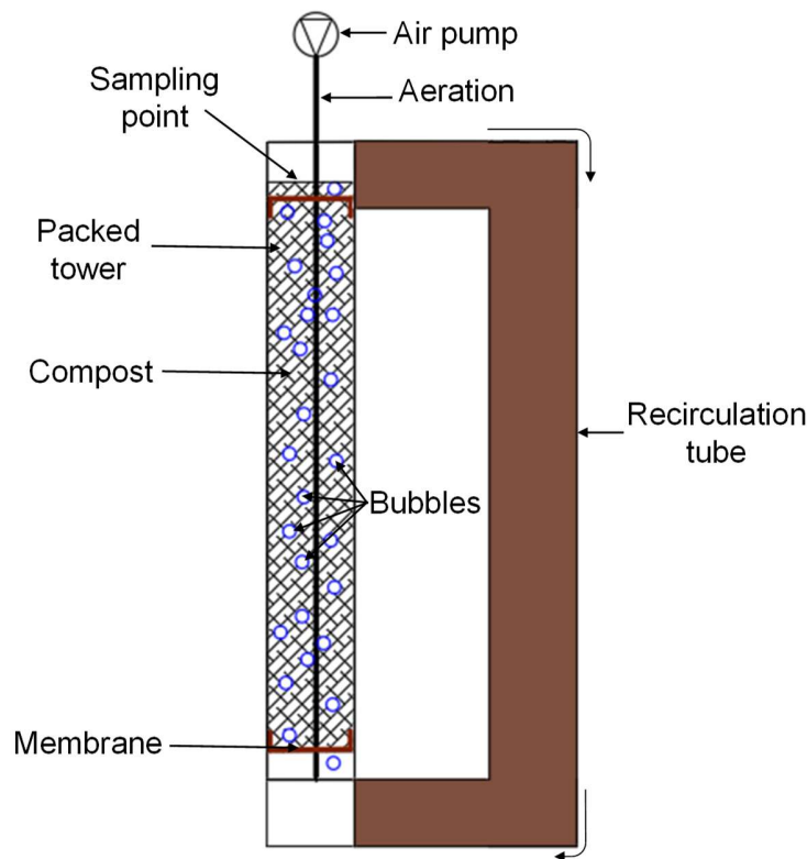
Figure 2. Schematic diagram of the airlift packing bioreactor (APBR).
