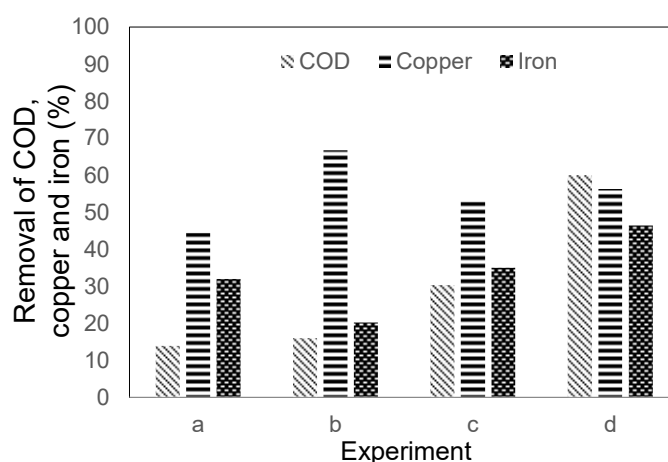
Figure 6. Removal of pollutants (%) present in LL treated in the APBRs, using a) raw LL, or different pretreatment processes: b) Coag/Floc, c) filtration and d) photo-Fenton).
