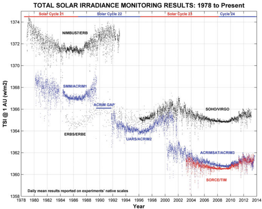
Fig. 33 Total solar irradiance recording by absolute radiometers in different space missions since 1978. Taken from www.acrim.com (as available in July/2018)
