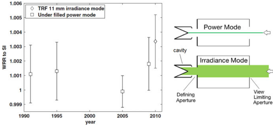
Fig. 32 (Left) Results of WRR to SI intercomparisons. Taken from Fehlmann et al. (2012). (Right) different operation modes for radiometers of the SI and WRR scales (power versus irradiance). Taken from Suter et al. (2012)
