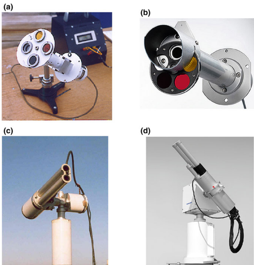
Fig. 29 Examples of filter radiometers based on rotating filter wheels and one (or two) sensors. a Eppley NIP pyrhelimeter with a manual 4-position filter wheel and three narrowband filters; b delta ohm LP PYRHE 16 with a 5-position filter wheel; c CIMEL 318 sun photometer, with 9 and 12 \lambda versions available, fully automated filter wheel, assembled in a two-axis sun tracker; d Kipp and Zonen POM-01 and POM-02 sky radiometers, also with fully automated 7 and 11 filters versions
