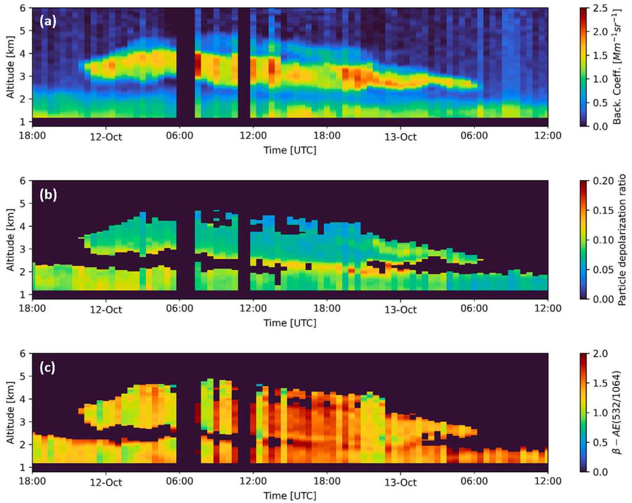
Fig. 5. Time series of particle properties observed by Raman lidar over Évora: (a) particle backscatter coefficient at 532 nm, (b) linear particle depolarization ratio and (c) backscatter-related Ångström exponent for the wavelength pair 532–1064 nm. The gaps in the layer (from 06:00 to 07:30 UTC and from 11:00 to 12:00 UTC on day 12) correspond to the periods where lidar retrievals were not possible due to the cloud presence.
