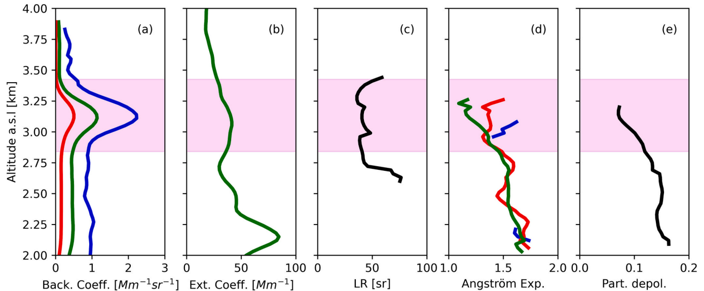
Fig. 8. The 1-h mean values of the VA optical properties derived from the Raman lidar measurements on 20 October from 04:00 to 05:00 UTC: (a) Particle backscatter coefficients (355 nm in blue, 532 nm in green and 1064 nm in red), (b) extinction coefficient at 532 nm, (c) lidar ratio at 532 nm, (d) backscatter related Ångström exponents (355–532 nm in blue, 532–1064 nm in green and 355–1064 nm in red) and (e) particle depolarization ratio at 532 nm. The volcanic aerosol layer between 2.8 km and 3.4 km asl is highlighted by the shadow area. (For interpretation of the references to colour in this figure legend, the reader is referred to the web version of this article.)
