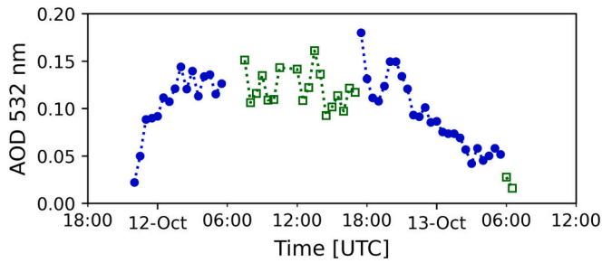
Fig. 7. Temporal series of the layer aerosol optical depth at 532 nm obtained by integrating the extinction coefficients from Raman lidar measurements (night time; blue circles) and the elastic backscatter coefficient and mean lidar ratio (day time; open green squares). (For interpretation of the references to colour in this figure legend, the reader is referred to the web version of this article.)
