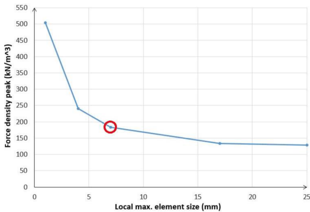
Fig. 23. Volumetric forces in the mid-upper interface of the IAM with the ISS at t=30 ms.
