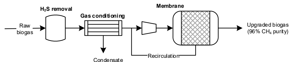
Figure 9. Scheme of membrane gas separation process. Adapted from Muñoz et al. [103].
