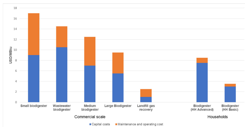
Figure 11. Investment and maintenance costs for biogas production technology per unit of energy produced in 2018. HH = household; “HH Advanced” includes pre-manufactured biogas digesters made of more expensive composite material; “HH Basic” includes biogas digesters constructed in place using traditional construction materials such as sand, gravel and cement. Adapted from [14].
