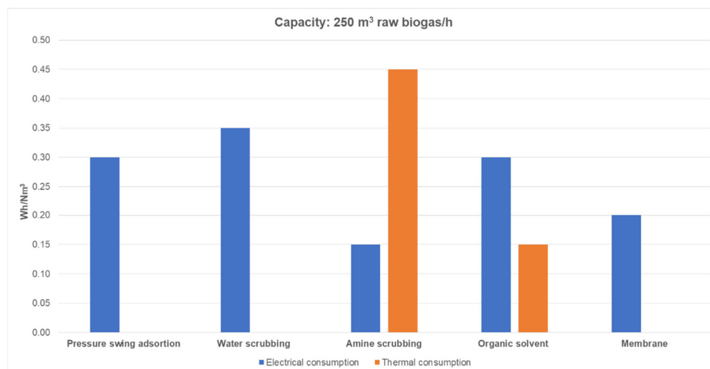
Figure 13. Energy and heat consumption by upgrading technology at 250 Nm³/h capacity plant. Adapted from Niederbacher [113].
