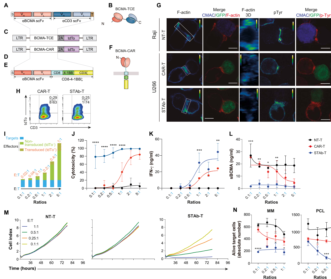
Fig. 1. BCMA-specific STAb-T cells show enhanced cytotoxic activity in vitro and promote canonical immunological synapses compared to CAR-T cells.
