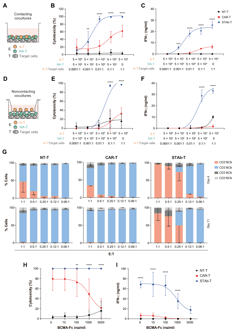
Fig. 2. STAb-T cells recruit bystander T cells and prevent tumor escape in vitro.
