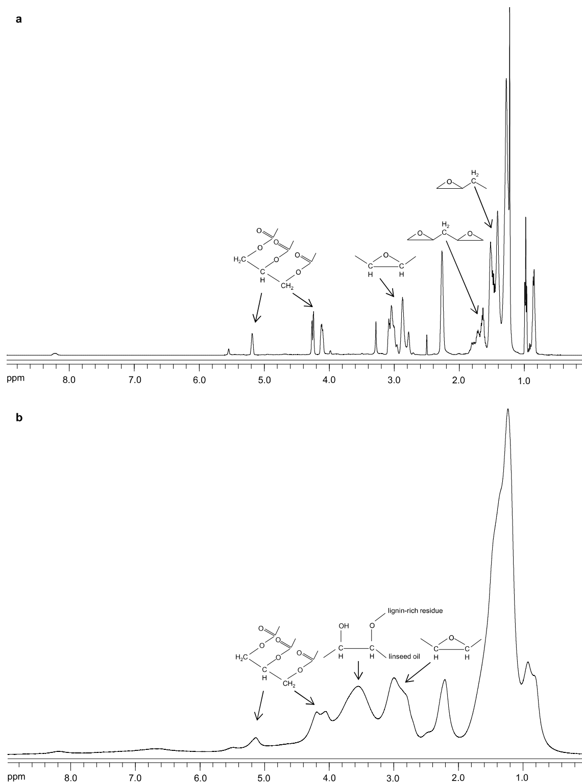
Fig. 4. ^1\text{H} NMR spectra of a epoxidized linseed oil (ELO) and b formulation obtained from OS lignin residues dispersed in ELO
