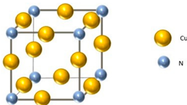
Figure 1. Picture of the anti- \text{ReO}_3 crystal structure of the \text{Cu}_3\text{N} compound. The copper atoms are represented by the yellow balls, and the nitrogen by the grey balls.
