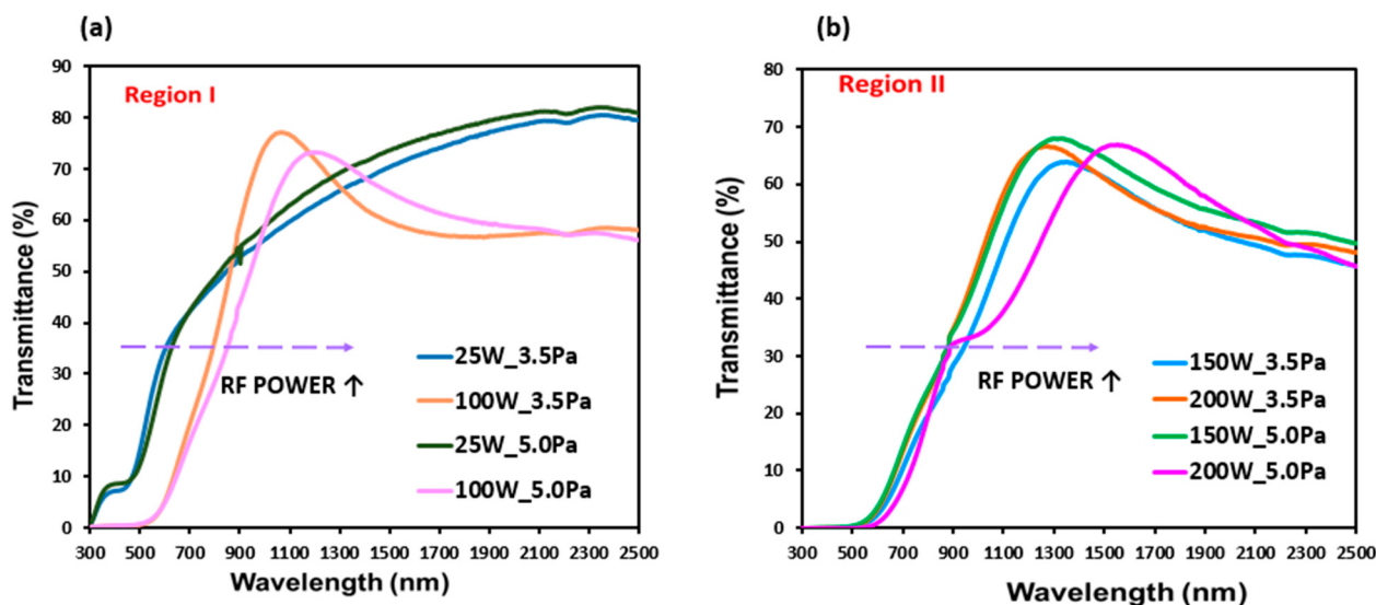
Figure 8. Transmittance spectra of Cu 3 N films prepared at different RF powers and working pressures. (a) region I; (b) region II.
