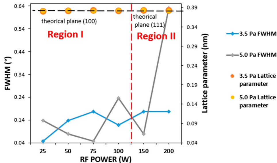
Figure 4. FWHM and lattice parameters extracted from the XRD spectra of \text{Cu}_3\text{N} films deposited at the gas pressures of 3.5 Pa and 5.0 Pa and the different RF powers of 25 W to 100 W (region I) and 150 W and 200 W (region II).
