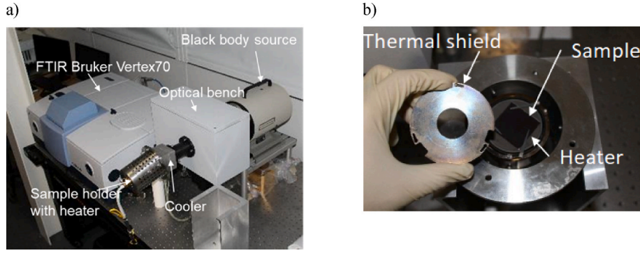
Fig. 4. CEA laboratory setup for spectral emittance measurements at operating temperature. a) Benchtop optical assembly. b) Sample holder overview.
