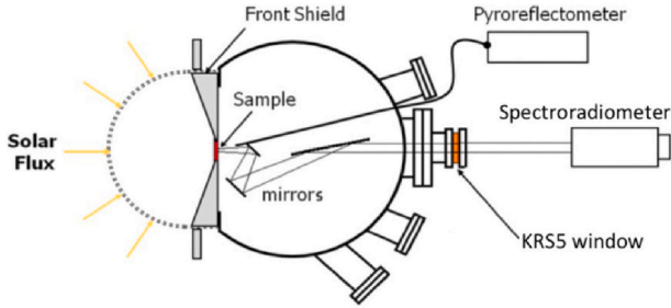
Fig. 5. MEDIASE setup mounted at the focus of the 1 MW solar furnace in Odeillo, France.
