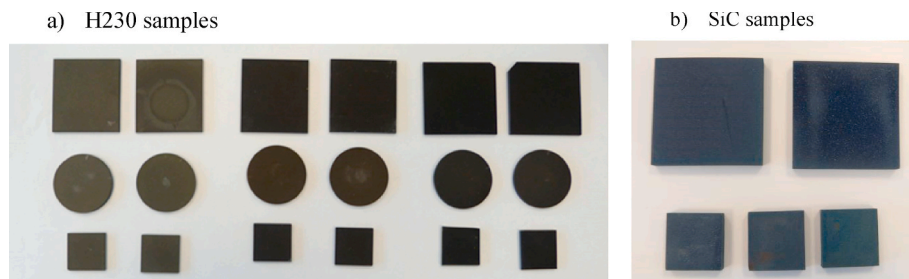
Fig. 1. a) H230 sample coupons submitted for RT and OT measurements. Samples are shown upon return after both RT and OT test campaigns. Top, from left to right: R01A, R01B, R02A, R02B, S1, S2. Middle, left to right: D01A, D01B, D02A, D02B, S3, S4. Bottom, left to right: A1, A2, B1, B2, S5, S6. b) SiC samples submitted for RT and OT measurements. Top: original samples. Bottom: Square inch samples cut by PROMES-CNRS for OT measurements up to 500 °C.
