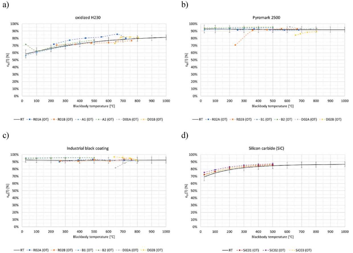
Fig. 17. Comparison of thermal emittance \epsilon_{th}(T) values for H230 and SiC sample coupons obtained from RT and OT measurements. a) oxidized H230, b) Pyromark 2500, c) Industrial grade black coating, d) SiC sample coupons.
