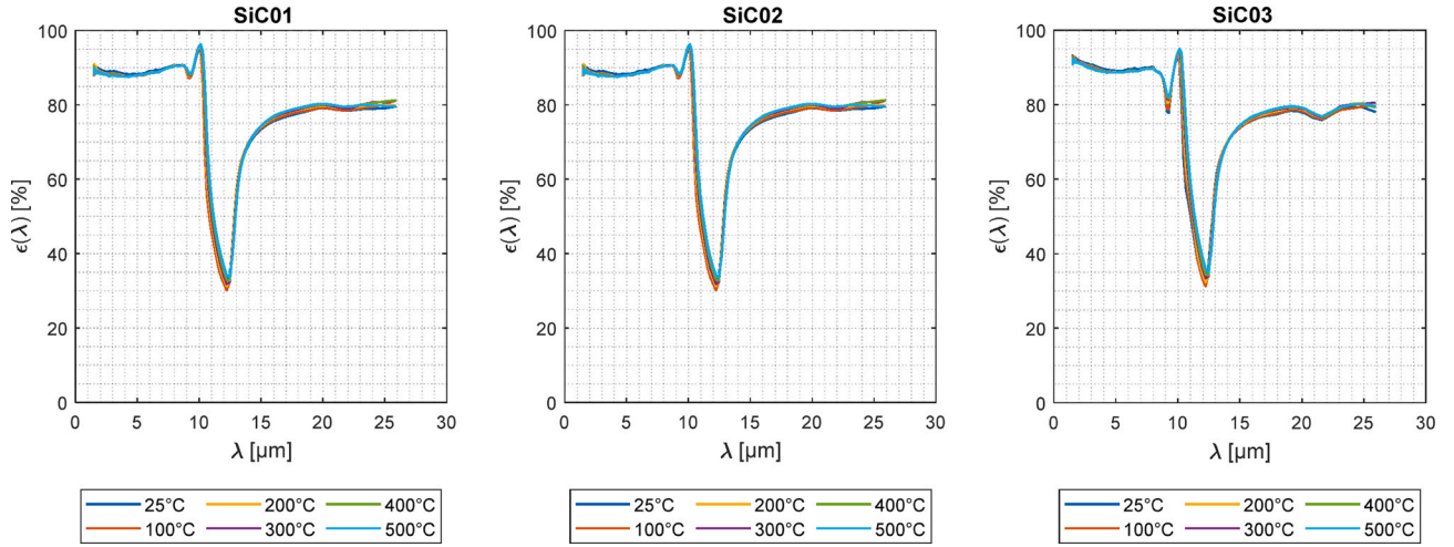
Fig. 14. Spectral measurements recorded for SiC sample coupons from 25 °C to 500 °C by PROMES-CNRS laboratory with the DTGS detector ( >1.5 \mu\text{m} ).
