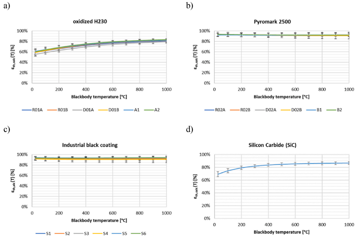
Fig. 8. Thermal emittance \varepsilon_{th,calc}(T) for H230 and SiC sample coupons (RT measurements). a) oxidized H230, b) Pyromark 2500, c) Industrial black coating, d) SiC sample coupons.
