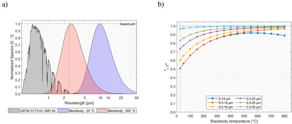
Fig. 6. a) Reference solar spectrum [31] and blackbody spectra at 25 and 800 °C. b) Fraction of Stefan-Boltzmann law ( f_{\sigma T^4} ) as a function of blackbody temperature for different spectral ranges.
