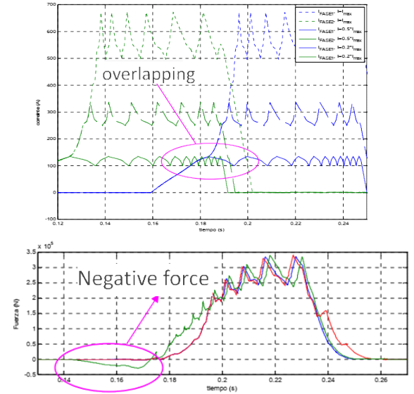
Fig. 13. Overlapping of machine phases and negative force: effects due to the non-appropriate selection of activation angles in AMSRG.
