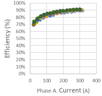
Fig. 12. Efficiency of the linear PTO.
