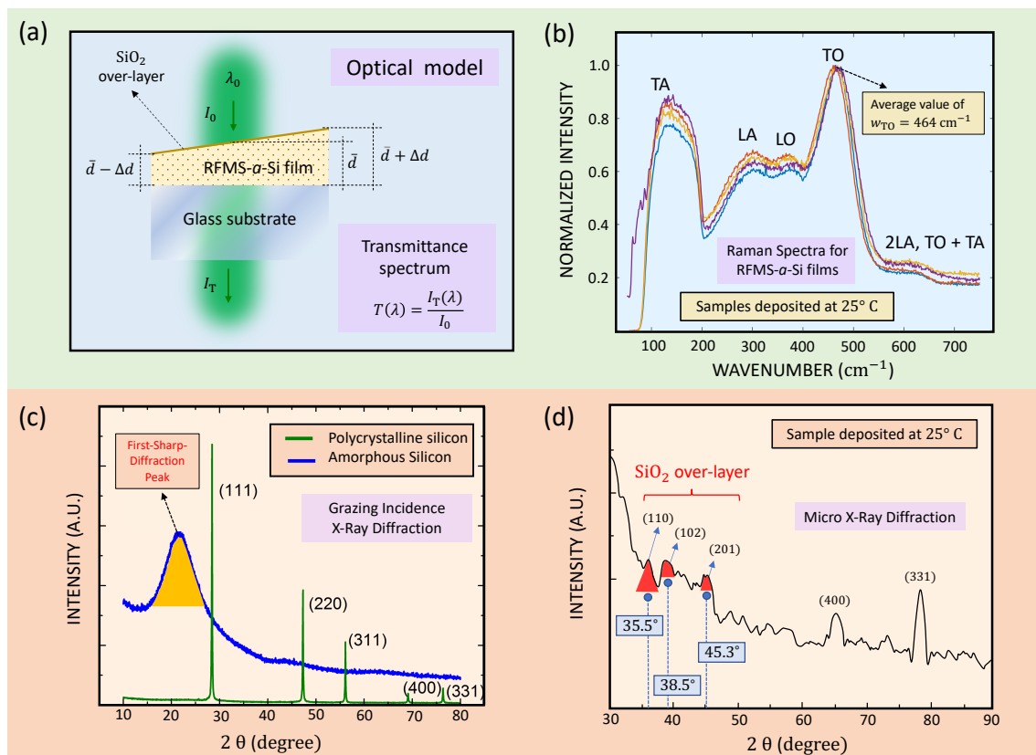
Figure 1. (a) A schematic illustration of the wedge-shaped geometry of a thin layer. (b) Raman spectra of four \alpha -Si specimens deposited at 25 °C [12,13]. (c) Grazing-incidence XRD diagram and (d) micro-XRD pattern of an \alpha -Si thin-film sample, grown at a temperature of 25 °C. In the micro-XRD diagram of this particular sample, several pronounced diffraction peaks can be noticed, which can be undoubtedly attributed to SiO 2 peaks (surface native oxide). The two diffraction peaks, (400) and (331), observed exclusively in this particular specimen, can correspond to crystalline planes of silicon indicative of a possible ordered nano-structure (nano-crystalline nature), embedded in the whole and absolutely dominant amorphous matrix (it has been considered negligible from the viewpoint of the assumed optical model) [14,15].
